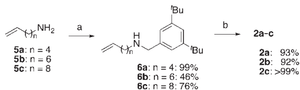
Scheme 3. Reagents and conditions: (a) 3,5-di- tert -butylbenzoic acid, EDCI·HCl (1-ethyl-3-(3-dimethylaminopropyl)-carbodiimide hydrochloride), DMAP, \text{CH}_2\text{Cl}_2 ; \text{LiAlH}_4 , THF, reflux and (b) HCl, MeOH; \text{NH}_4\text{PF}_6 , acetone.
