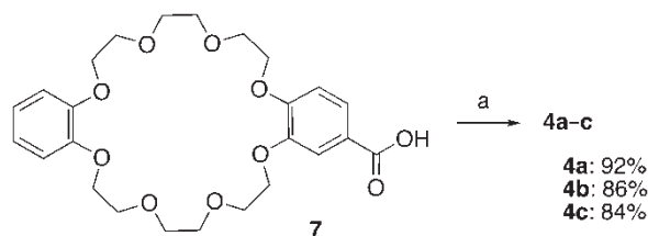
Scheme 4. Reagents and conditions: (a) diol, EDCI·HCl, DMAP, \text{CH}_2\text{Cl}_2 . Diol is 4a for 1,4-butanediol, 4b for 1,6-hexanediol and 4c for 1,8-octanediol.
